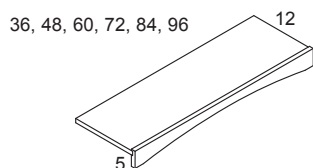
Roman Arch Canopy Valance - RACV • The Canopy Valance may have the front substituted with the Roman Arch, or the Arched Raised Panel Valances. Shown here with Roman Arch option. • Arch height is 3" at center.
