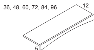
Roman Arch Canopy Valance - RACV • The Canopy Valance may have the front substituted with the Roman Arch, or the Arched Raised Panel Valances. Shown here with Roman Arch option. • Arch height is 3" at center.
