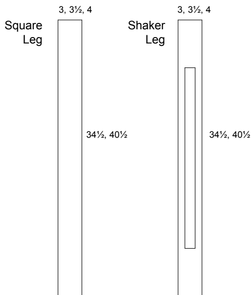
Leg Cutting Options
